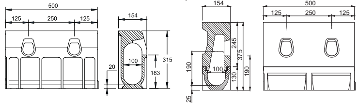
MEAKERB 320 drainage channel body | MEAKERB 320 BS drainage channel body
